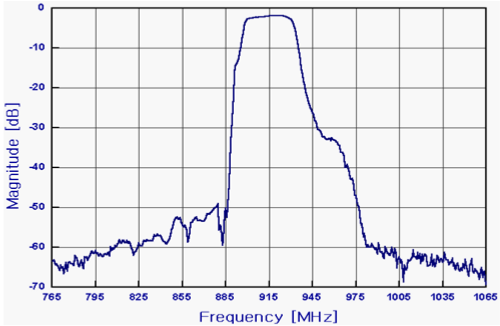
Frequency Response
