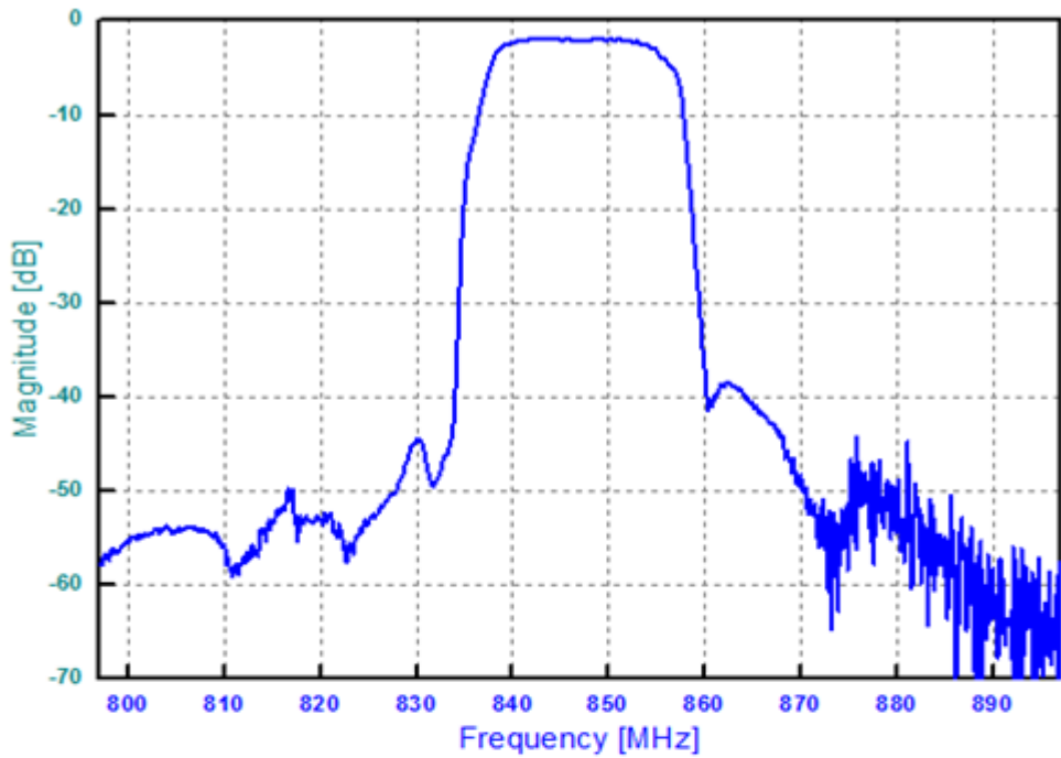
Frequency Response
