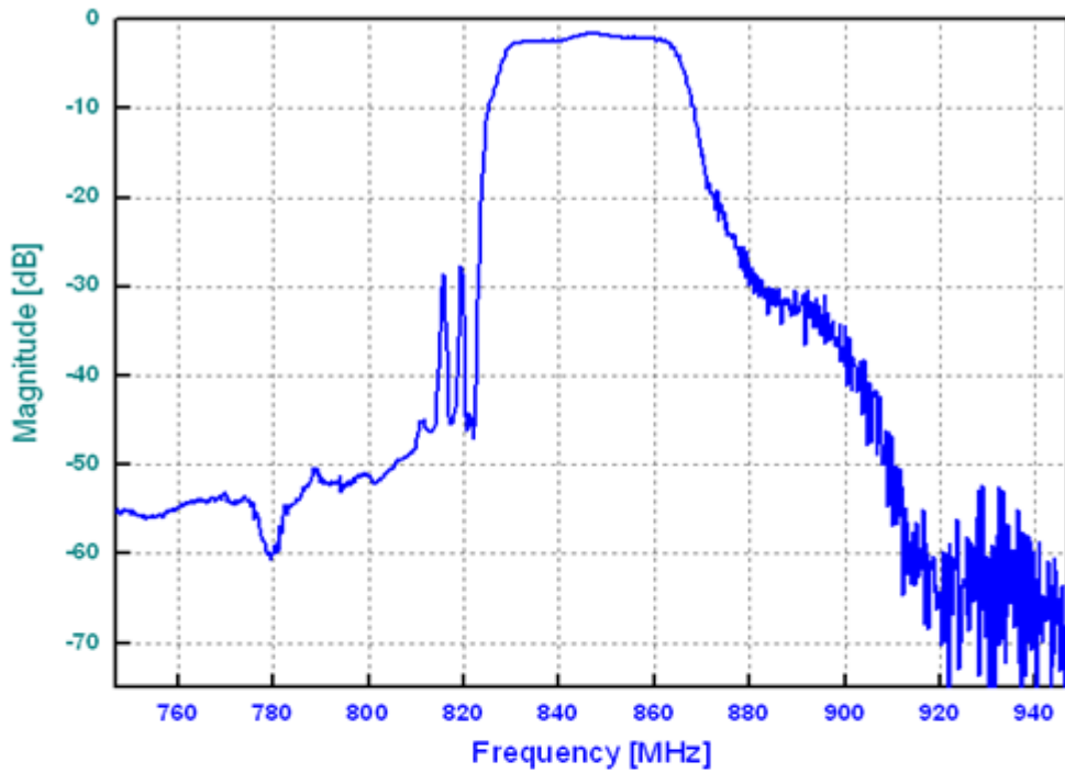
Frequency Response
