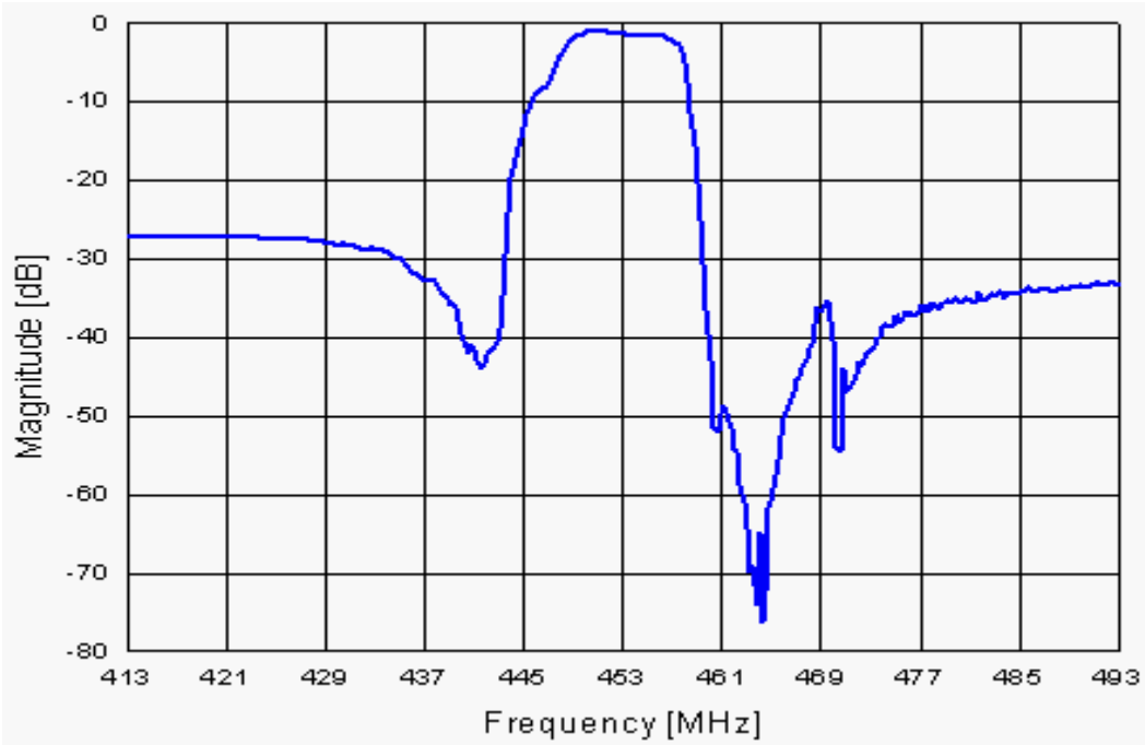
Frequency Response
