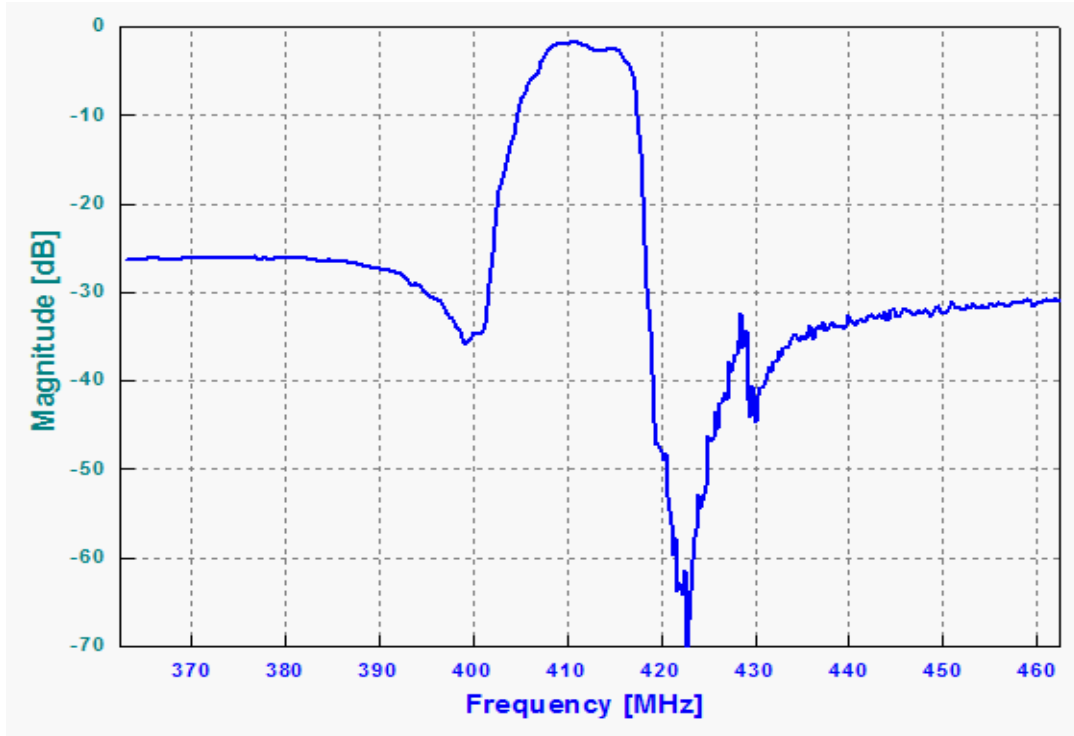
Frequency Response
