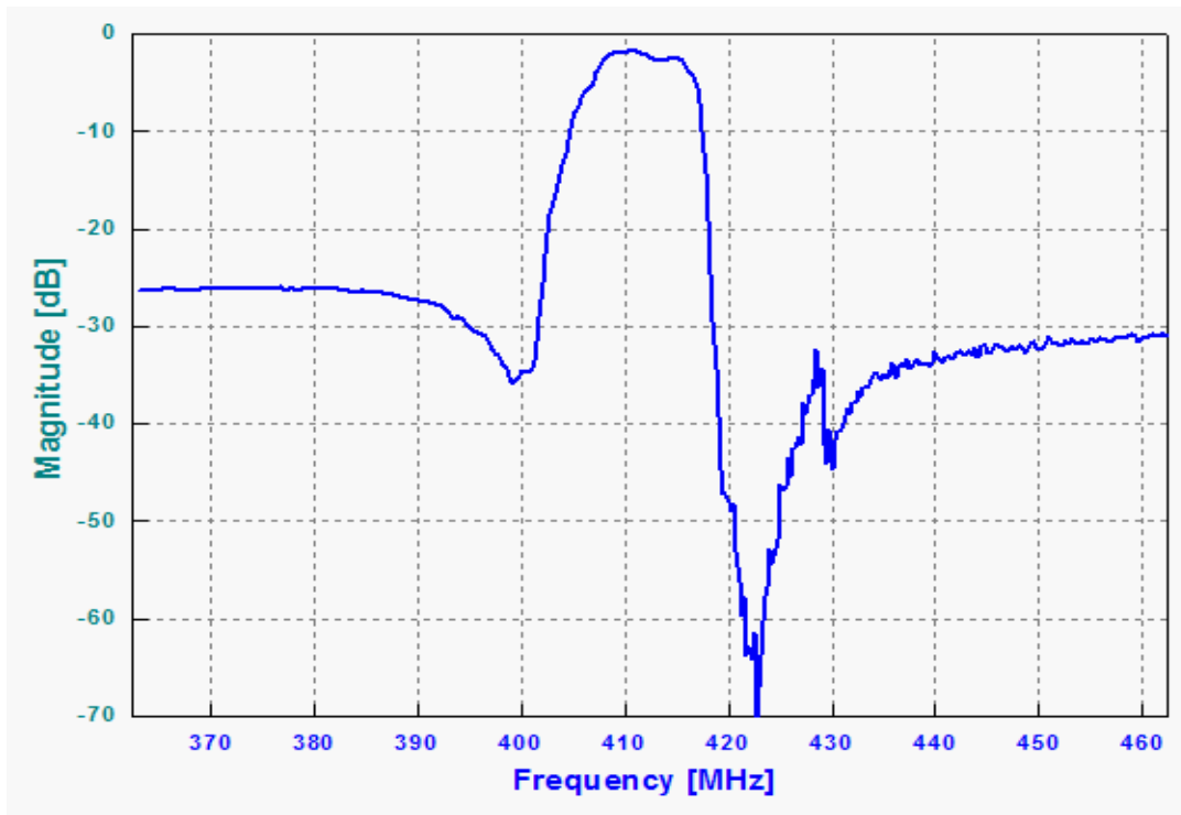
Frequency Response
