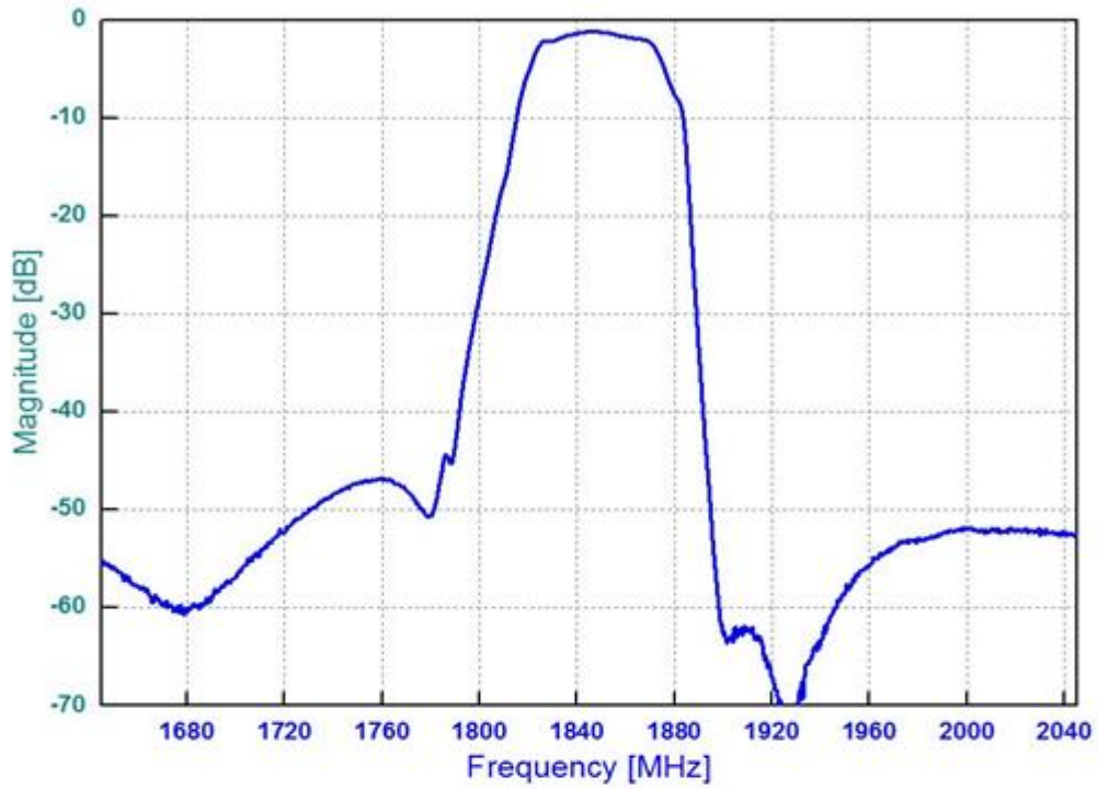
Frequency Response
