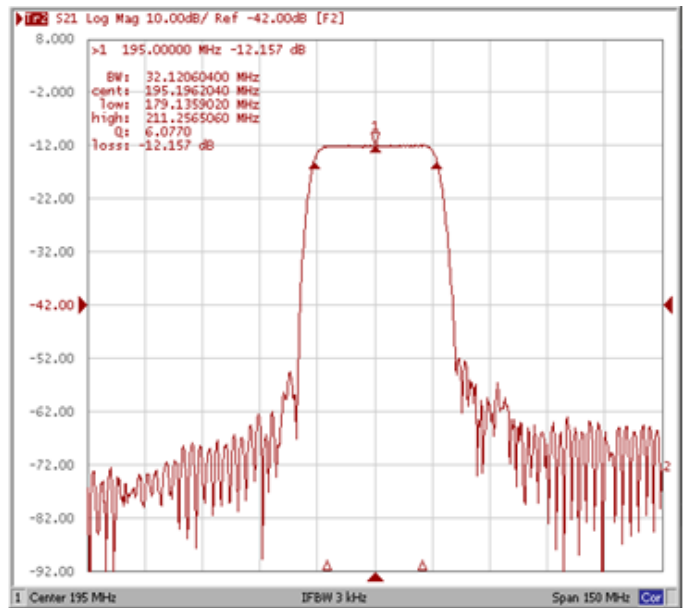
Attenuation Fo ± 35.00 MHz/ Fo ± 40.00 MHz
