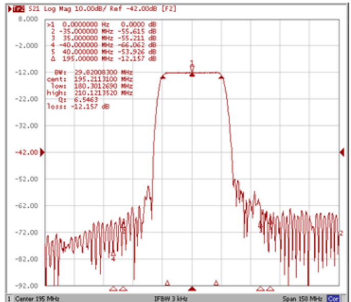
Attenuation Fo ± 35.00 MHz/ Fo ± 40.00 MHz
