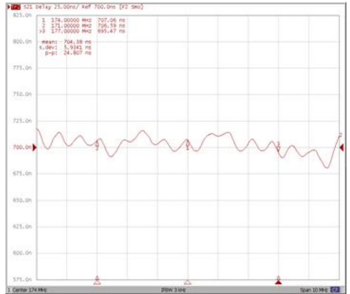
Group Delay Variation at Fo±3.0MHz
