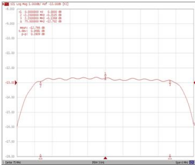
Ripple Variation Fo±2.2MHz
