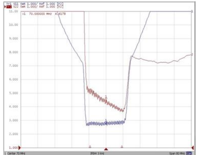
SWR
