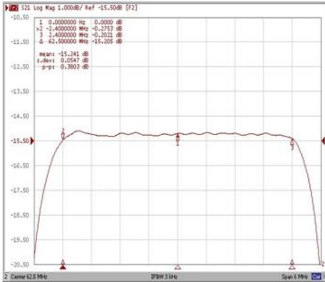
Ripple Variation Fo±2.40MHz
