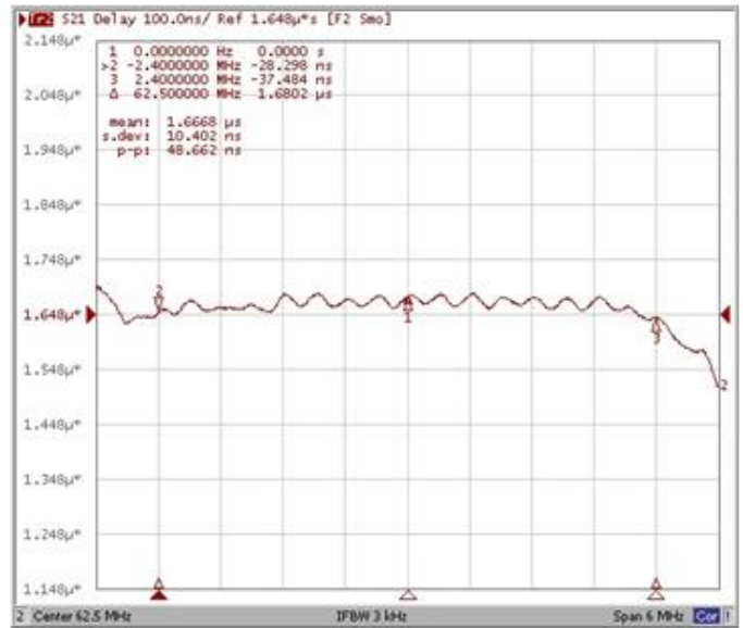
Group Delay Variation Fo±2.40MHz
