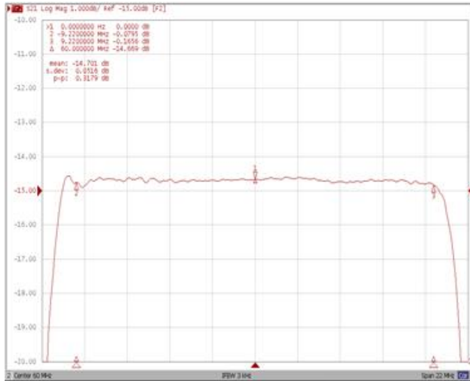
Ripple Variation Fo±9.22MHz
