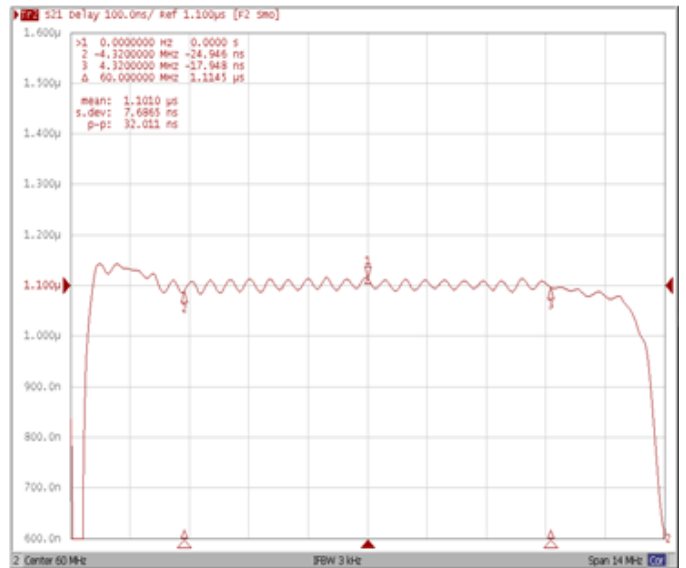
Group Delay Variation Fo±4.32MHz
