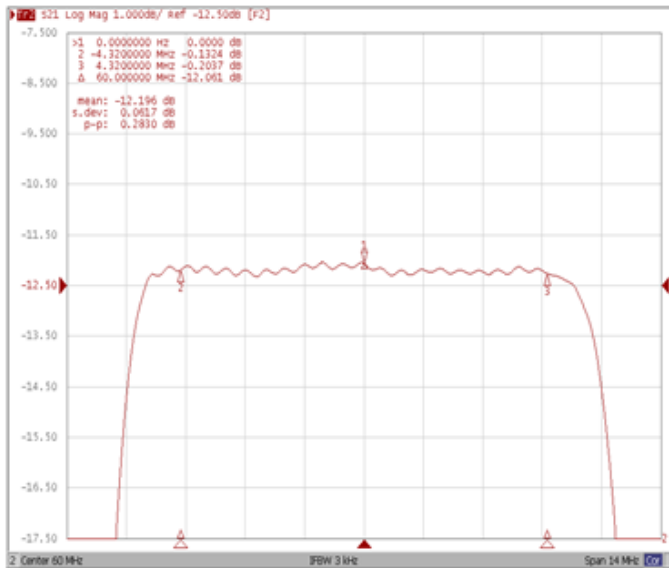
Ripple Variation Fo±4.32MHz
