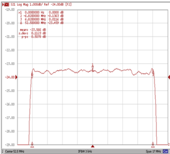
Ripple Variation Fo±6.82MHz
