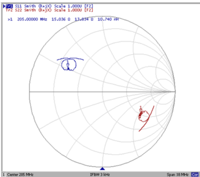
Smith Chart
