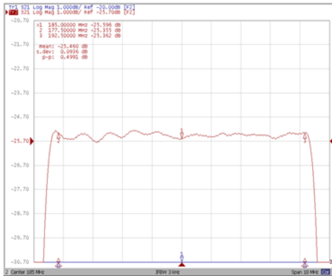
Ripple Variation Fo \pm 7.5\text{MHz}
