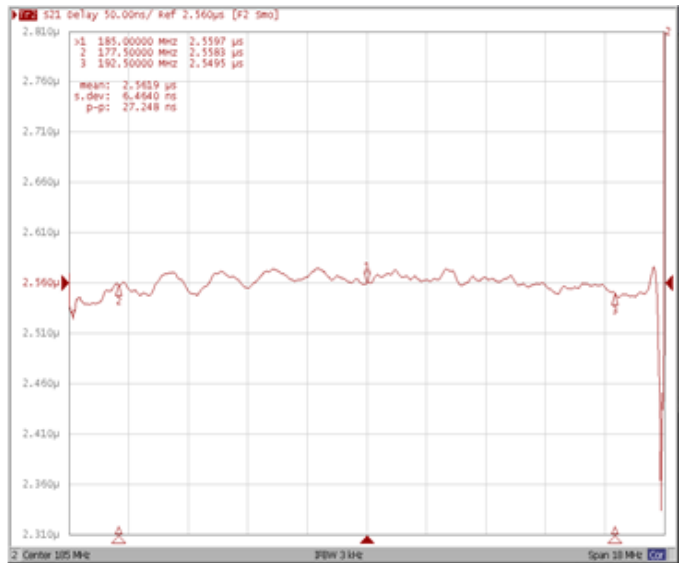
Group Delay Variation Fo \pm 7.5\text{MHz}
