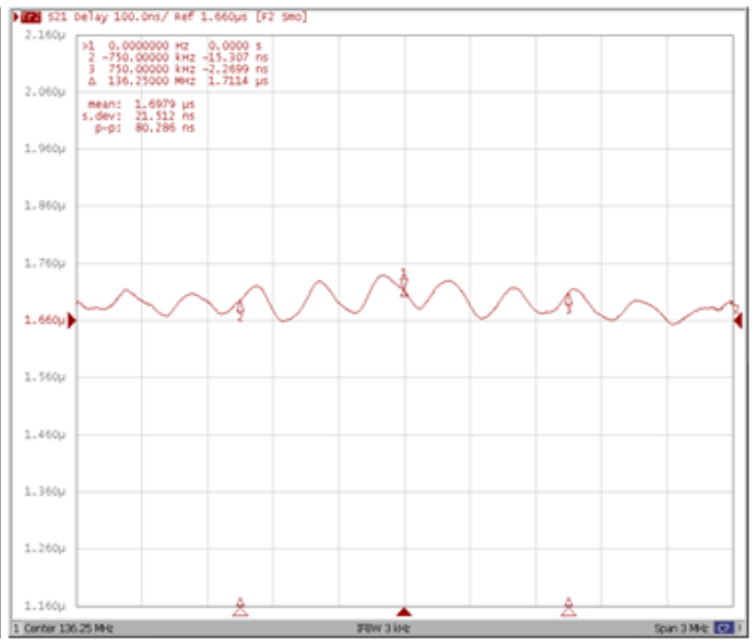
Group Delay Variation Fo±0.75MHz
