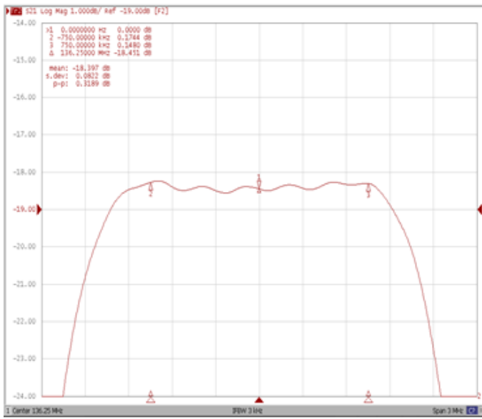
Ripple Variation Fo±0.75MHz
