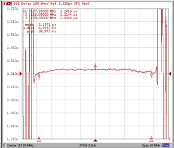
Group Delay Variation F_0 \pm 11.50\text{MHz}
