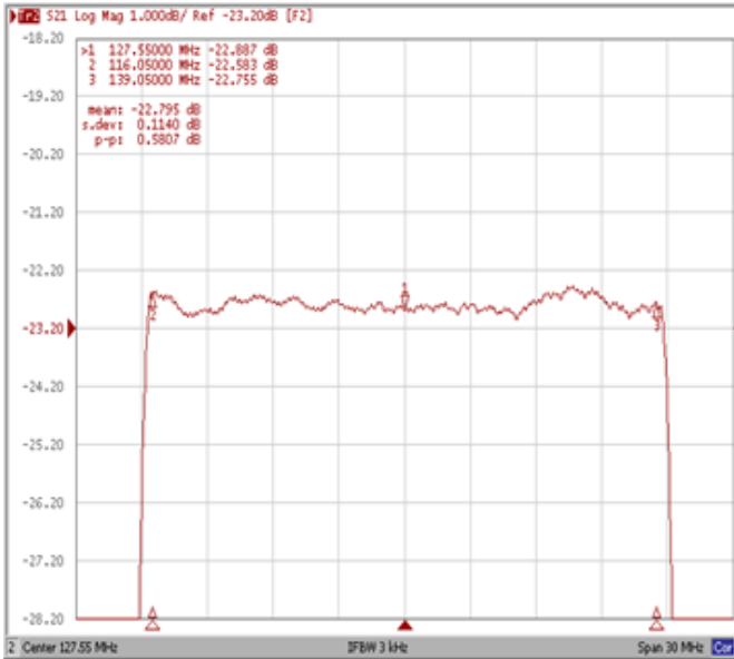
Ripple Variation F_0 \pm 11.50\text{MHz}
