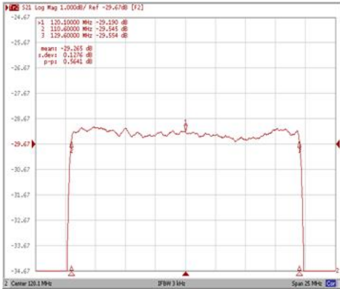
Ripple Variation Fo±9.5MHz
