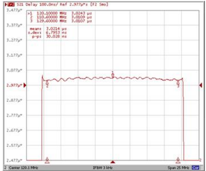
Group Delay Variation Fo±9.5MHz
