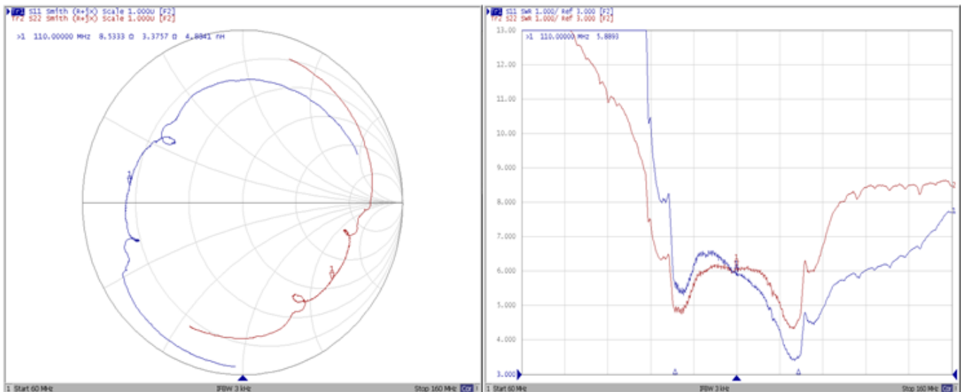
Smith Chart
