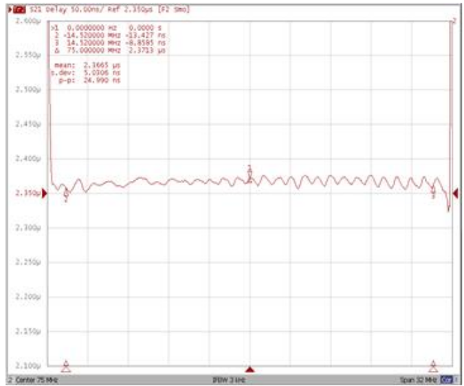
Group Delay Variation Fo±14.52MHz
