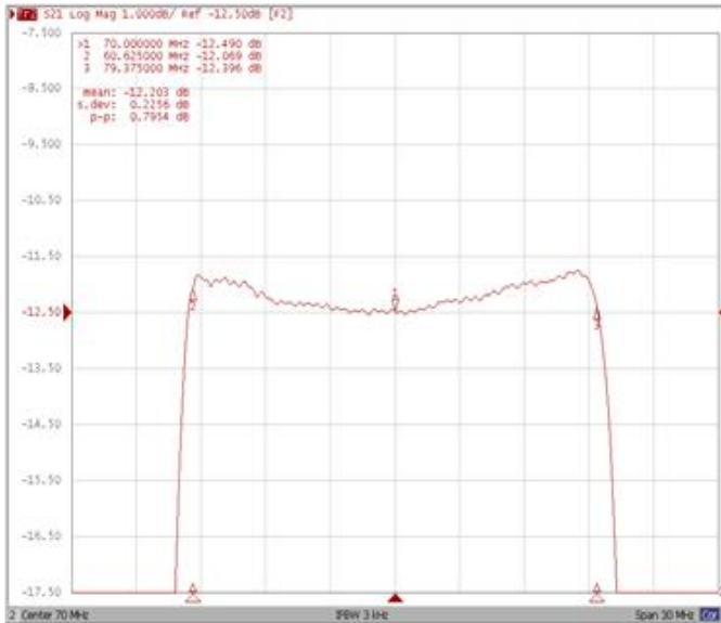
Ripple Variation Fo±9.375MHz
