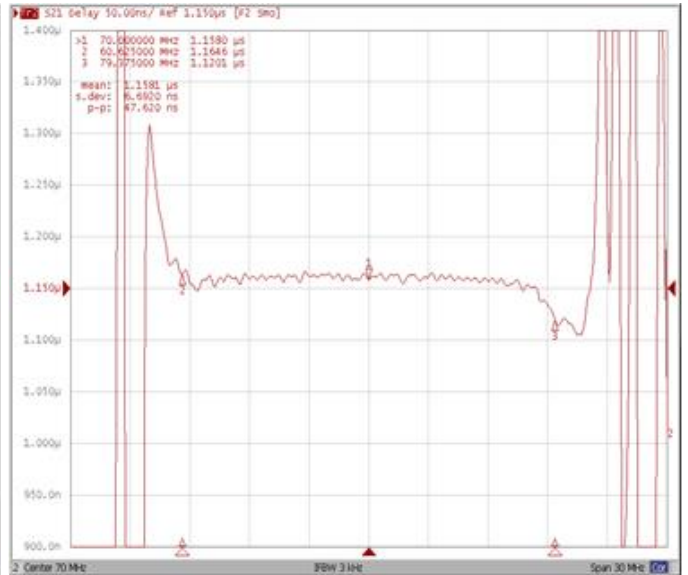
Group Delay Variation Fo±9.375MHz
