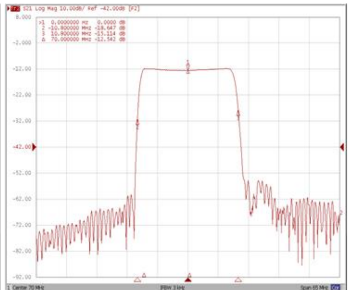
Relative Attenuation F_{0\pm 10.8\text{MHz}}
