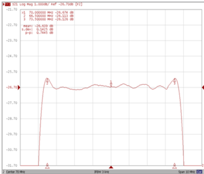
Ripple Variation Fo±3.50MHz
