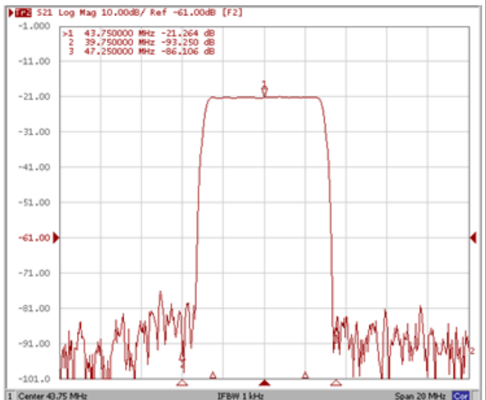
Attenuation 39.75 / 47.25MHz
