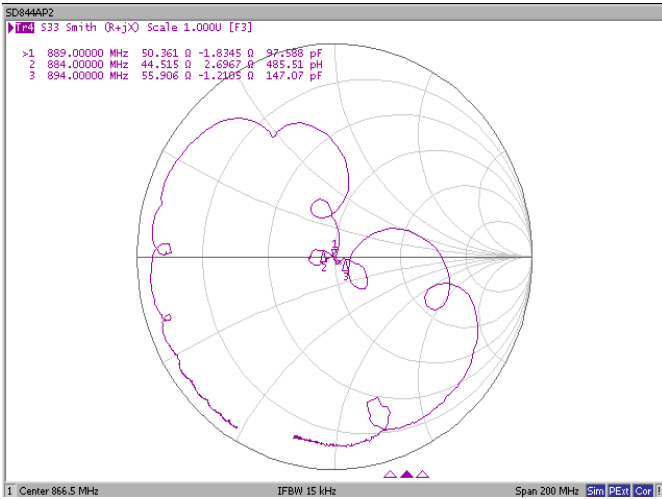
Smith Chart
