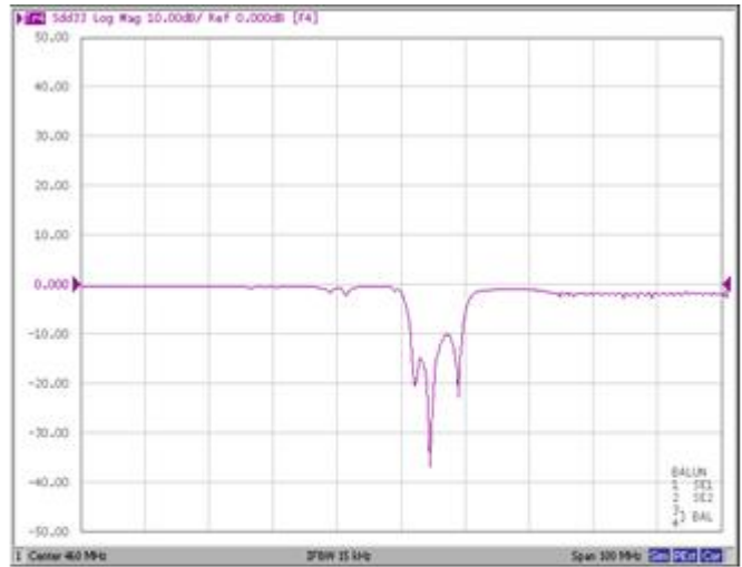
Return Loss
