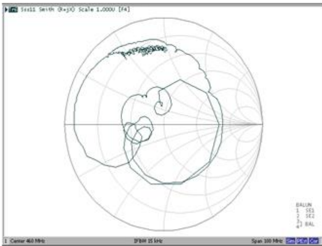
Smith Chart
