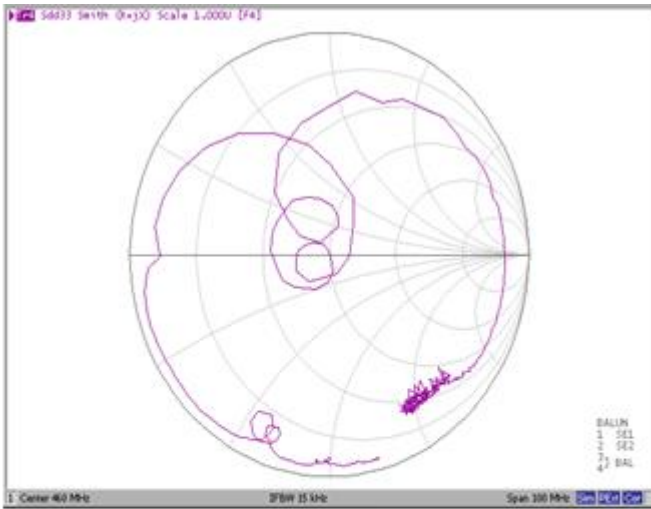
Smith Chart
