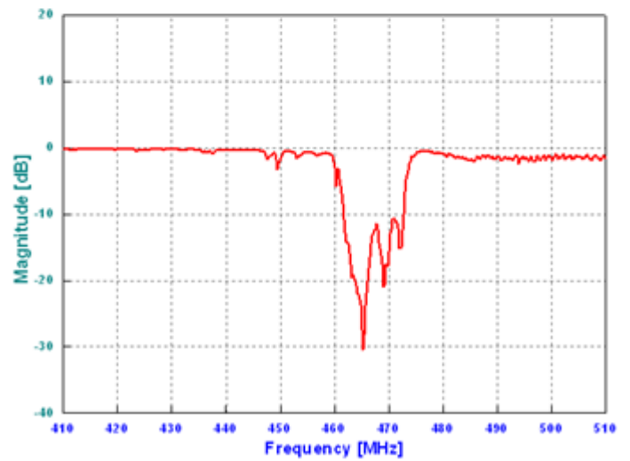
Return Loss
