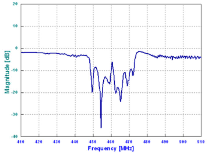
Return Loss
