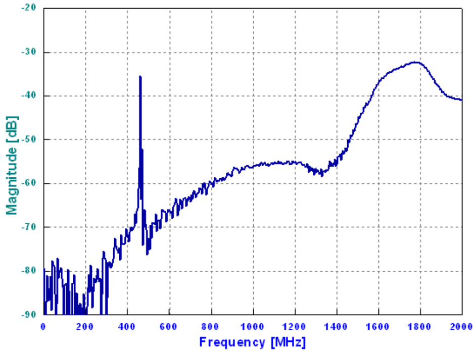
Tx to Rx Isolation Wide Band
