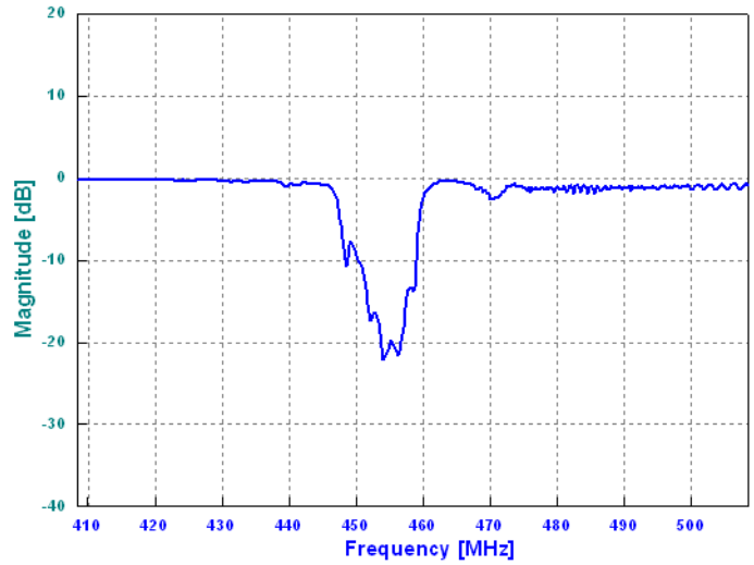
Return Loss
