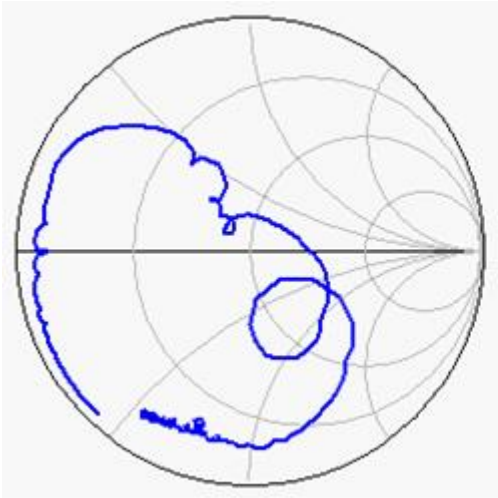
Smith Chart
